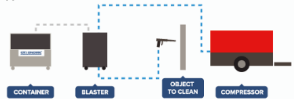
CLEANING OBJECTS WITH DRY ICE
